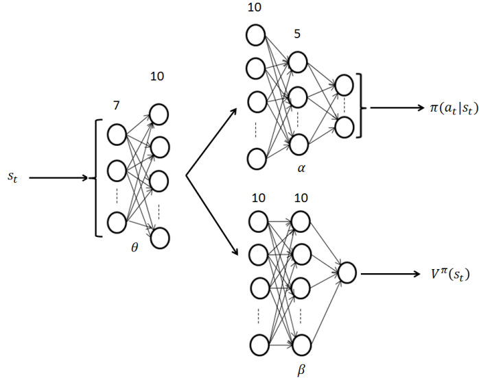
Fig. 4: The employed dueling network architecture with shared parameters \theta . \alpha and \beta are the actor- and critic-specific parameters, respectively. All the layers are fully connected neural networks; the numbers shown above represent the hidden layer dimensions. The policy network on the upper branch estimates the action probabilities via a softmax output layer, while the critic network on the lower branch approximates the state-value function.
