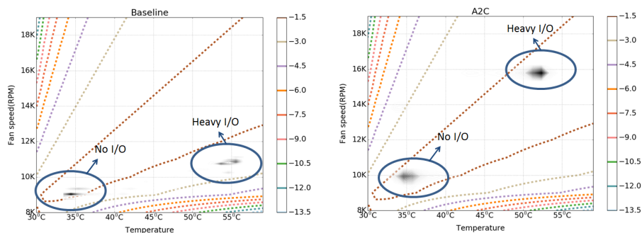
Fig. 7: For the no load scenario, the baseline policy settles to 36^{\circ}\text{C} and 9K rpm while the A2C algorithm converges to 35^{\circ}\text{C} and 10K rpm. With heavy I/O loading, the corresponding numbers are 55^{\circ}\text{C} and 11K versus 52^{\circ}\text{C} and 16K. The A2C algorithm is seen to always settle at the innermost contour, as desired.
